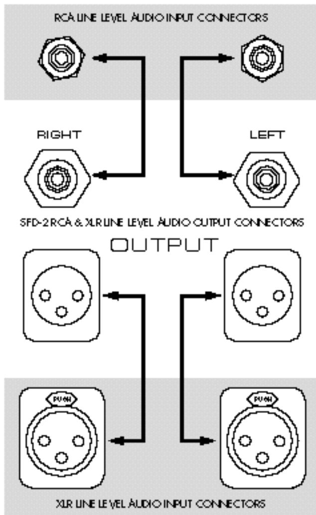
Figure 4- The SFD-2 XLR balanced and RCA single-ended audio output connections to a line level amplification device - right channel to right channel and left channel to left channel. Both the XLR and RCA output connections can be hooked up in unison, although this setup would be system dependent.
