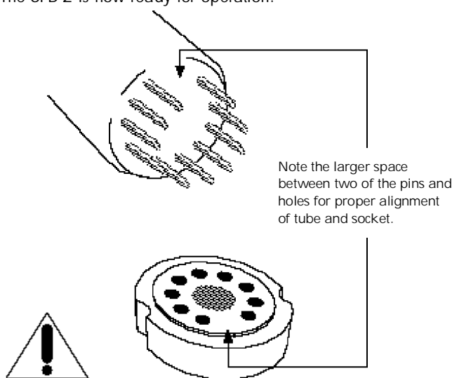
Figure 2 - Tube pin alignment with the socket.
