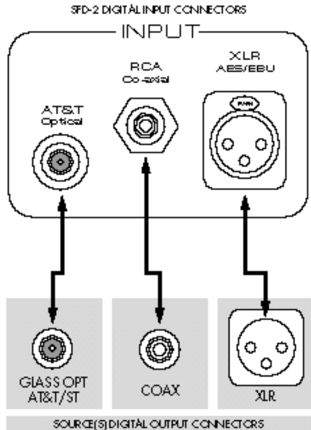
Figure 3- The digital source(s) output connections to the SFD-2 digital inputs. Up to three digital sources may be connected to the SFD-2 Digital Processor via AT&T/ST Glass Optical, Coaxial RCA and AES/EBU XLR interconnect.
